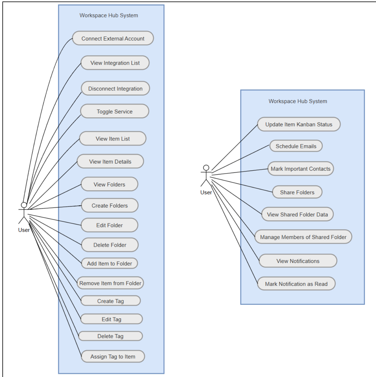
Use case diagram - User
